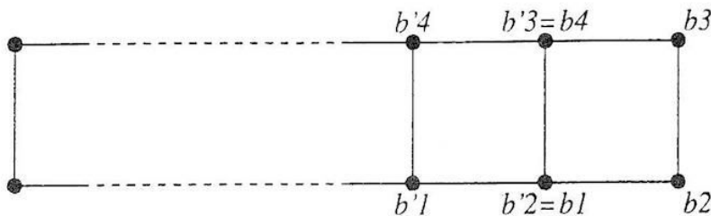
Ladder graph.
