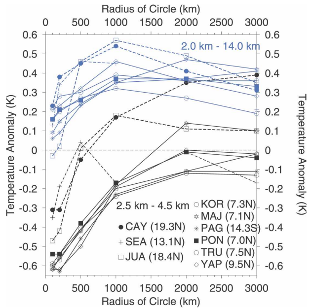
FIG. 5. The convective temperature anomaly (black curves), averaged between 2.5 and 4.5 km, plotted against the radius of the circle within which rainfall is enhanced. Dashed curves refer to radiosonde stations in the Caribbean. The spatial extent of the lower-tropospheric cooling is much larger in the equatorial Pacific than in the Caribbean. The blue curves show the full-depth tropospheric temperature anomaly between 2.0 and 14.0 km. The full-depth warming is slightly larger in the Caribbean than in the equatorial Pacific. The correspondence between the three-letter codes and radiosonde stations is the same as in Fig. 4.
