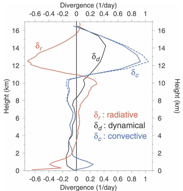
FIG. 6. The dynamical divergence is an average of all divergence profiles from the IFA array during TOGA COARE. The radiative divergence is an annual mean profile calculated from radiosonde temperature and relative humidity profiles from Koror (7.4°N). The convective divergence \delta_c was calculated from the formula \delta_c = \delta_d - \delta_r . The dashed blue curve is the convective divergence profile obtained by setting the cloud fraction equal to zero at all heights.
