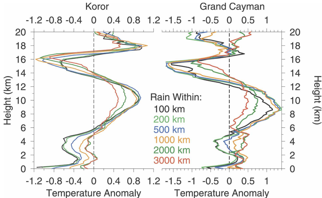
FIG. 1. (left) The temperature anomaly at Koror ( 7.3^{\circ}\text{N} ), averaged over times in which the instantaneous average rainfall rate within circles of various radii centered at Koror is in the top 10% for that month. The temperature anomaly is defined with respect to the monthly mean. (right) The convective temperature anomaly profiles at Grand Cayman ( 19.3^{\circ}\text{N} ).
