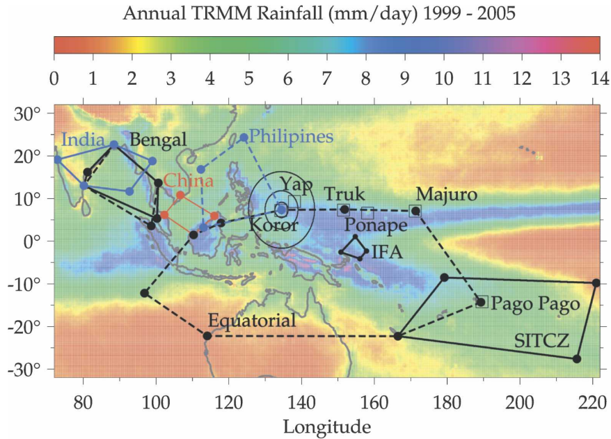
FIG. 2. A map showing the various rawinsonde arrays used to calculate the dynamical divergence profiles, superimposed on annual mean TRMM rainfall (1999–2005). The arrays have been drawn in different colors to help distinguish them from each other—India: blue, Bay of Bengal: solid black and dashed black, South China Sea: red, Philippines: dashed blue, equatorial: dashed black, SITCZ: solid black, and IFA: solid black. Six of the high-resolution U.S. radiosonde stations are denoted by open boxes: Koror, Yap, Truk, Ponape, Majuro, and Pago Pago. The circles centered on Koror have radii equal to 500 and 1000 km.
