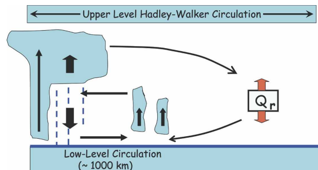
FIG. 11. A schematic plot of the thermodynamic forcings associated with the upper-level Hadley–Walker circulation and the shallow downdraft circulation.
