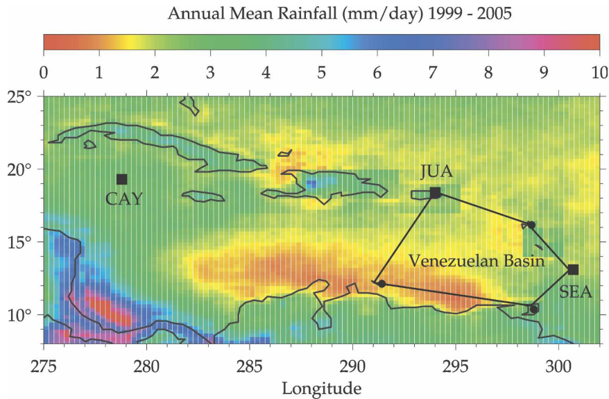
FIG. 3. A map of the Venezuelan Basin array superimposed on TRMM annual mean rainfall. The squares indicate the locations of the U.S. high-resolution radiosonde sites.
