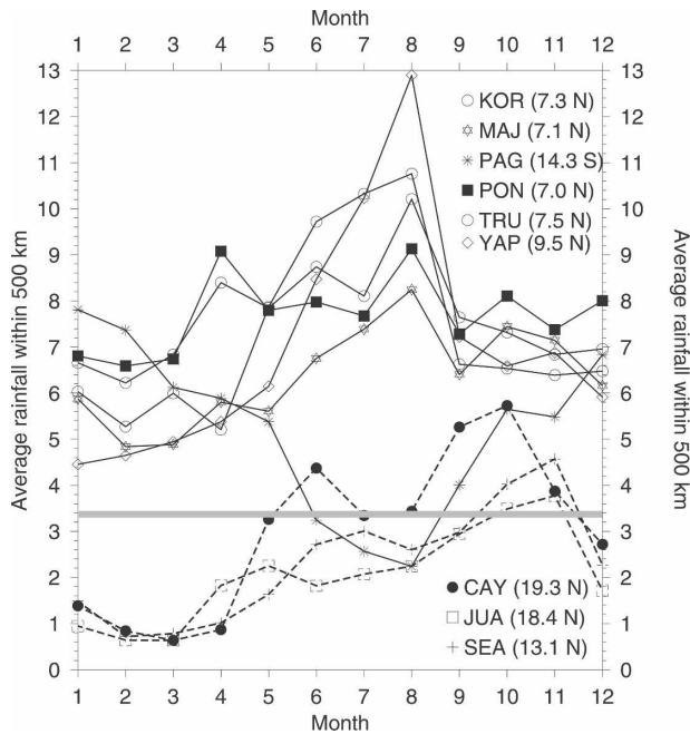
FIG. 4. The monthly mean rainfall rate within a circle with radius of 500 km centered at various islands. Rainfall rates were obtained from the TRMM 3B42 gridded rainfall product. The dashed curves refer to sites in the Caribbean. The horizontal gray line indicates the 3.4 mm day -1 rainfall threshold used in the calculation of the temperature anomaly profiles. Each location has been identified by a three-letter code—CAY: Grand Cayman, JUA: San Juan/Isla Verde (U.S.), KOR: Koror/Palau Island, MAJ: Majuro/Marshall Island, PAG: Pago Pago International Airport (Samoa), PON: Ponape Island, SEA: Seawell (Barbados), TRU: Truk International/Moen Island, and YAP: Yap Island.
