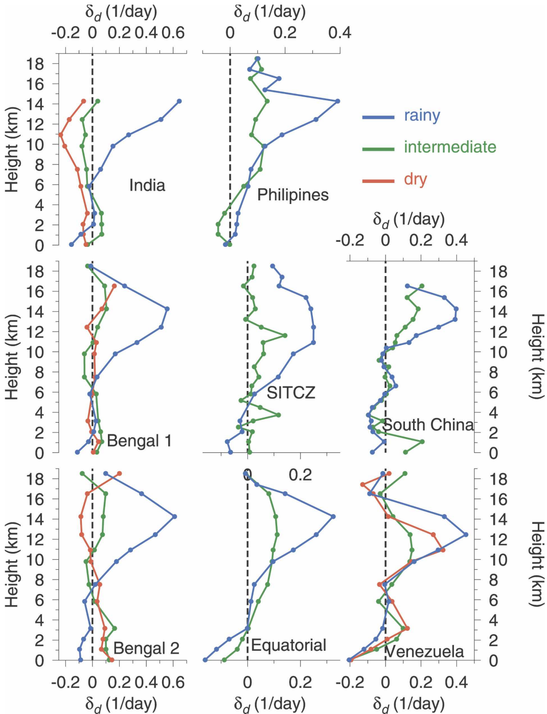
FIG. 7. Dynamical divergence profiles calculated from the rawinsonde arrays shown in Figs. 2 and 3. The rainy profiles shown in blue refer to averages over months in which the mean rainfall exceeded some threshold (usually 6 \text{ mm day}^{-1} ). Profiles shown in red refer to averages over months in which the mean rainfall was less than 1.5 \text{ mm day}^{-1} . Profiles shown in green refer to averages in which the monthly mean rainfall rate was larger than 1.5 \text{ mm day}^{-1} but less than the rainy threshold.
