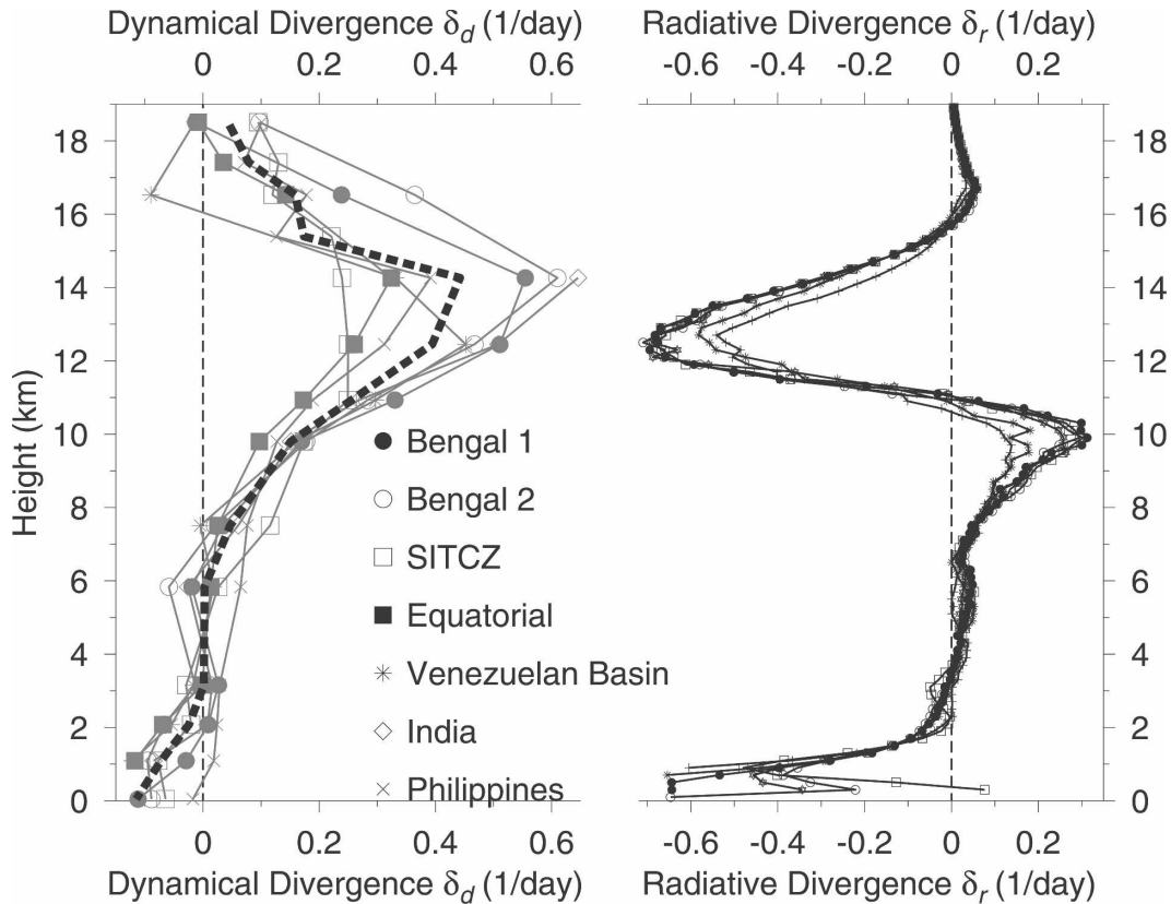
FIG. 9. (left) Seven of the eight rainy divergence profiles shown in Fig. 7 (South China is not shown since it has a size <1000 km). The thick dashed line is an average of all seven rainy divergence profiles. (right) The annual mean radiative mass flux divergence \delta_r profiles at five equatorial Pacific radiosonde stations: Koror, Truk, Majuro, Yap, and Ponape.
