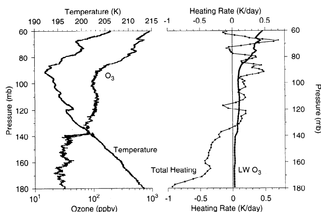
Figure 7. (left) Temperature and ozone, as measured from the ER-2 during the October 23 descent into Fiji, between 60 and 180 mbar. (right) Total (solar + longwave) clear sky heating rate versus pressure as calculated by a radiative transfer model using as inputs the ER-2 measurements of temperature, pressure, ozone, and water vapor. The contribution of the 9.6 \mu\text{m} ozone band to the total heating is shown as a thick line. Note the strong anticorrelation between temperature and heating rate near the tropopause. Photon path lengths in the 15 \mu\text{m} band of \text{CO}_2 are sufficiently short that positive temperature fluctuations are rapidly damped by negative heating rates, and vice versa.
