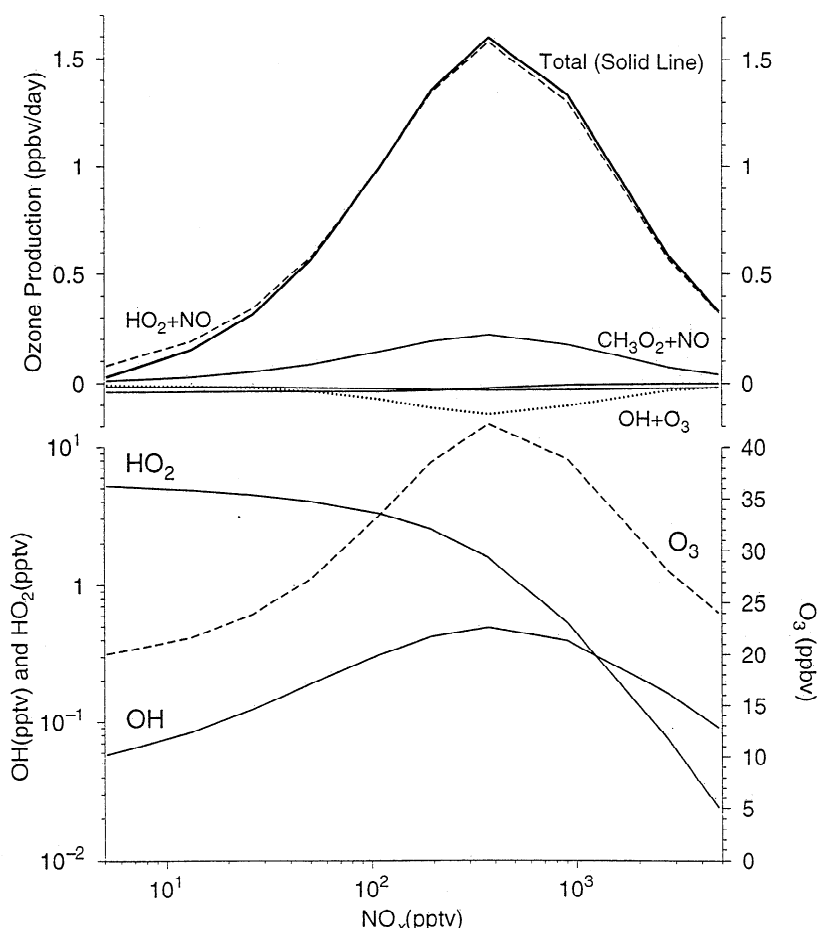
Figure 1. (bottom) Mixing ratios of OH in parts per trillion by volume (pptv), \text{HO}_2 (pptv), and \text{O}_3 (ppbv) in the baseline model run plotted against \text{NO}_x . (top) Ozone production and destruction terms in the baseline model run plotted against \text{NO}_x . The two small unlabeled ozone destruction terms are \text{OH} + \text{O}_3 and \text{O}^1\text{D} + \text{H}_2\text{O} . The dashed line represents ozone production from the \text{HO}_2 + \text{NO} reaction. The dotted line represents destruction from the \text{HO}_2 + \text{O}_3 reaction. The bold line represents the sum of all five production and destruction terms.
