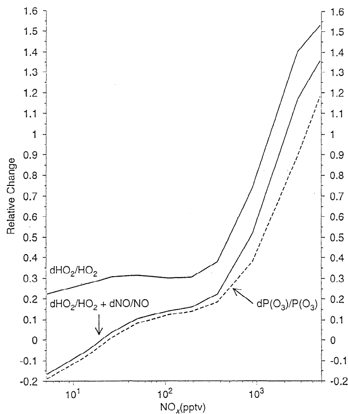
Figure 8. The fractional change in ozone production from adding acetone to the model (dashed line). Fractional changes in \text{HO}_2 , and in \text{HO}_2 + d\text{NO}/\text{NO} (solid lines).
