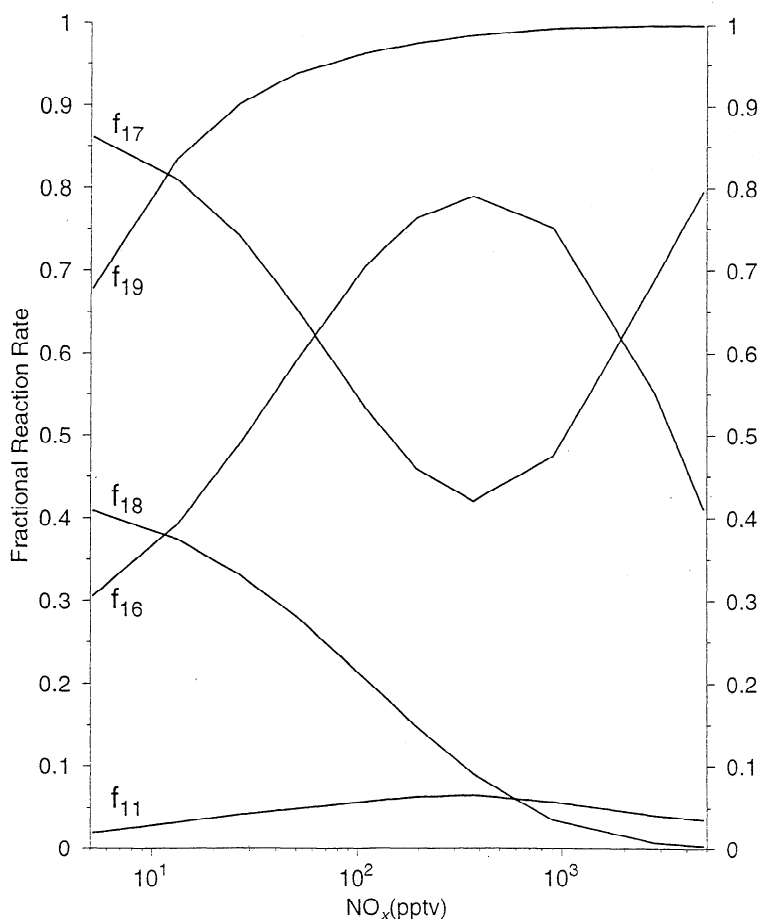
Figure 3. The dependence against \text{NO}_x of five fractional reaction rates: f_{17} , fraction of \text{HNO}_3 undergoing photolysis; f_{19} , fraction of \text{HO}_2 reacting with \text{NO} ; f_{18} , fraction of \text{NO} reacting with \text{HO}_2 ; f_{16} , fraction of \text{HNO}_4 reacting with \text{OH} ; and f_{11} , fraction of \text{CH}_3\text{COO}_2 reacting with \text{NO}_2 .
