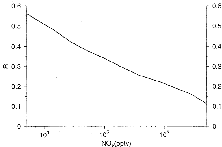
Figure 11. The variation with \text{NO}_x of the \text{HO}_x - \text{NO}_x coupling coefficient R as defined by equation (21) in the text.
