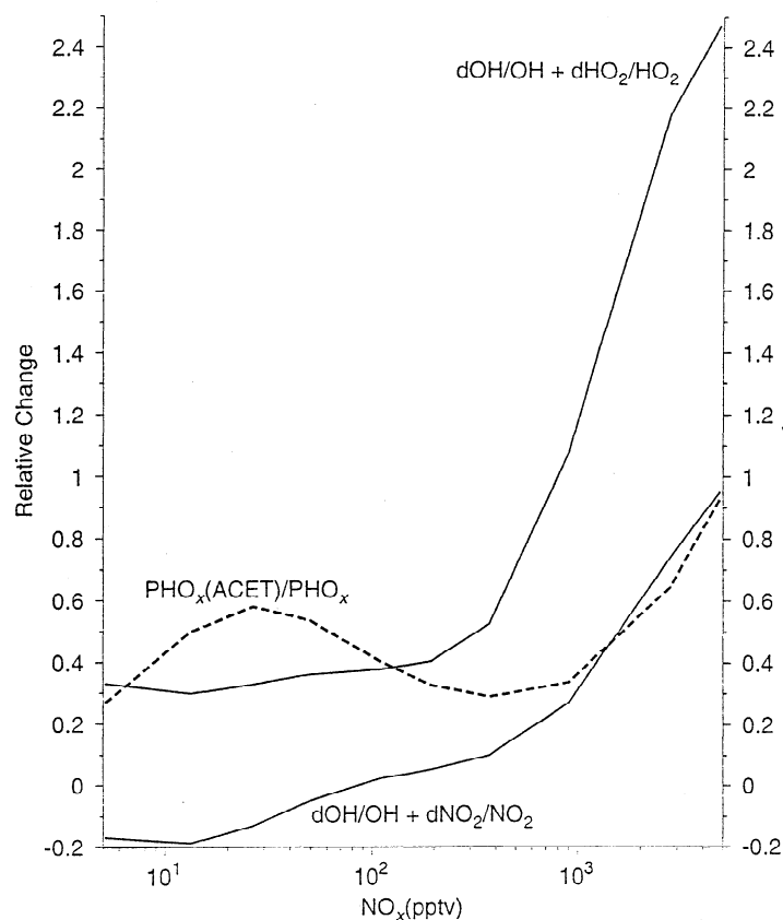
Figure 7. The dotted line represents the production of \text{HO}_x from acetone, normalized by the total production of \text{HO}_x in the baseline model. The two solid lines represent the sum of the fractional changes in OH and \text{HO}_2 and in OH and \text{NO}_2 .
