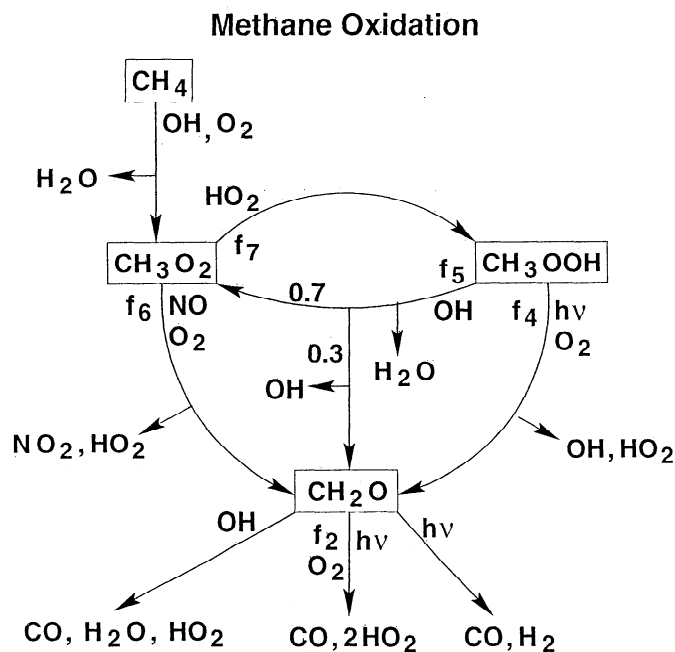
Figure 13. An overview of methane (CH 4 ) oxidation.
