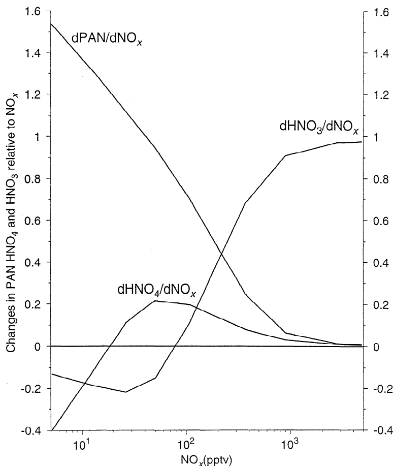
Figure 10. The changes in PAN, \text{HNO}_4 , and \text{HNO}_3 from the introduction of acetone, normalized by the absolute change in \text{NO}_x .
