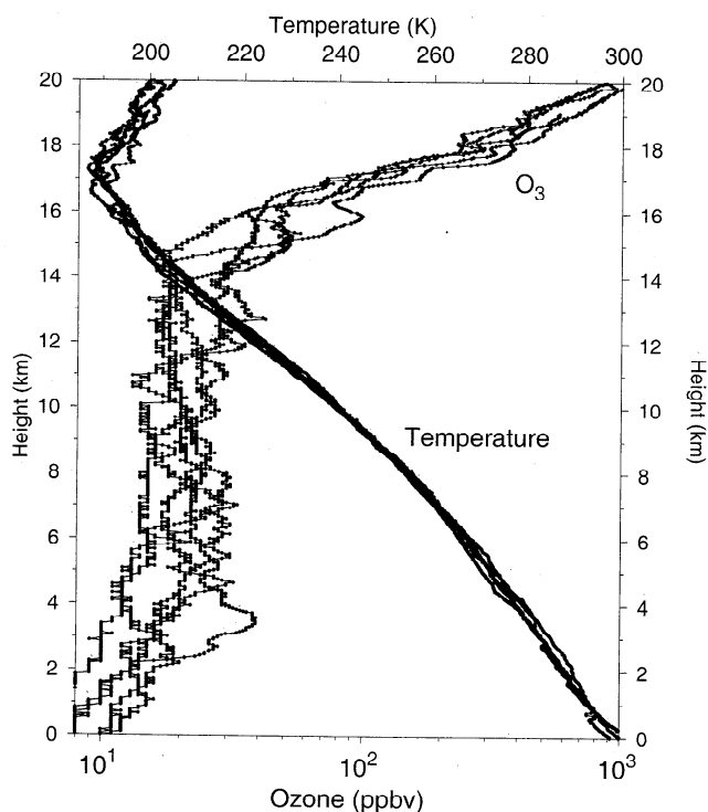
Figure 1. Profiles of temperature and \text{O}_3 taken from five ozonesondes launched from Samoa in March 1996.
