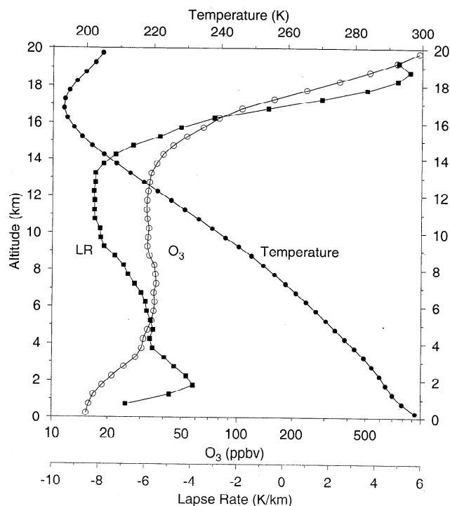
Figure 2. Average profiles of temperature, \text{O}_3 , and lapse rate (LR) from all 108 Samoan ozonesondes.
