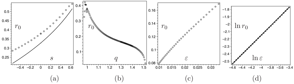
Figure 3. Experiment 2: The effect of parameter s on the smoke-ring radius with (p, q, m) = (2, 1, 2) and \epsilon = 0.04 . Dots indicate the radius obtained with direct numerical computation of (1.4) using FlexPDE. The solid line is obtained by solving for r_0 from formula (1.10). (b) Experiment 3: The effect of q with (p, m, s) = (2, 2, 0) and \epsilon = 0.04 . A smoke-ring solution exists for 1 < q < 1.5 . For 0.97 < q < 1 , FlexPDE has a hard time converging and the solution seems to jump around; FlexPDE fails to converge when q \leq 0.97 . (c) Experiment 4: The effect of \epsilon with (p, m, s) = (2, 2, 0) and q = 1.2 . (d) Experiment 4 on a log-log plot. The data is shown by circles; the line shows a straight-line fit r_0 \approx 1.51\epsilon^{0.64} through the last two points of the data.
