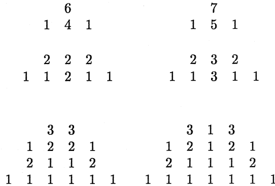
Figure 1: Creating palindromes of n = 6 and n = 7
