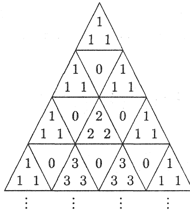
Figure 2: Palindromes with i parts
