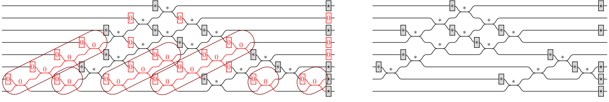
Figure 5.11: An example of a PPRS triangular normal form. In the figure on the left, the beam splitters and phase shifters with angle 0 in the corresponding triangular form are shown in red. In the figure on the right, they are replaced with identities.
