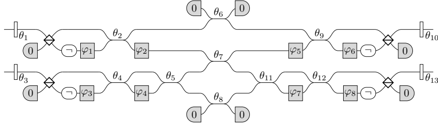
Figure 5.2: \text{LO}_v -circuit implementing a variational quantum eigensolver [110], an algorithm with applications including calculation of ground-state energies in quantum chemistry.
