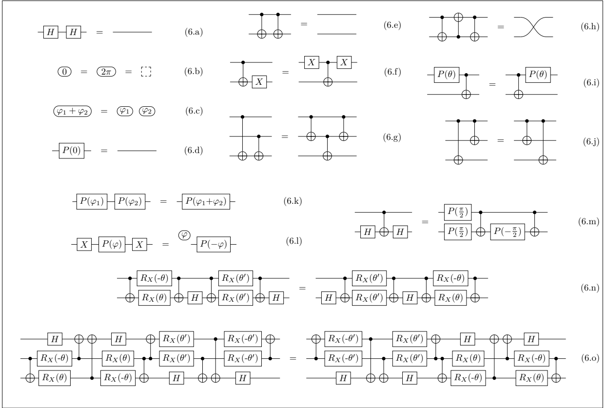
Figure 6.2: Axioms of \mathbf{QC}_0 : Structural equations on quantum circuits. The equations are defined for any \varphi, \varphi_1, \varphi_2, \theta, \theta' \in \mathbb{R} .
