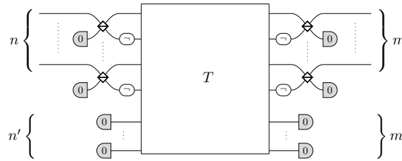
Figure 5.13: Shape of a circuit in normal form as of Definition 5.38.
