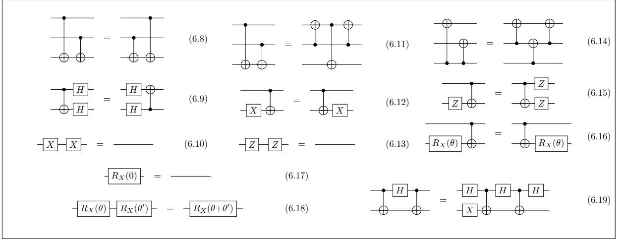
Figure 6.3: Standard circuit identities that can be derived from the axioms of \text{QC}_0 , given in Figure 6.2 . The proofs are given in Appendix D.1.
