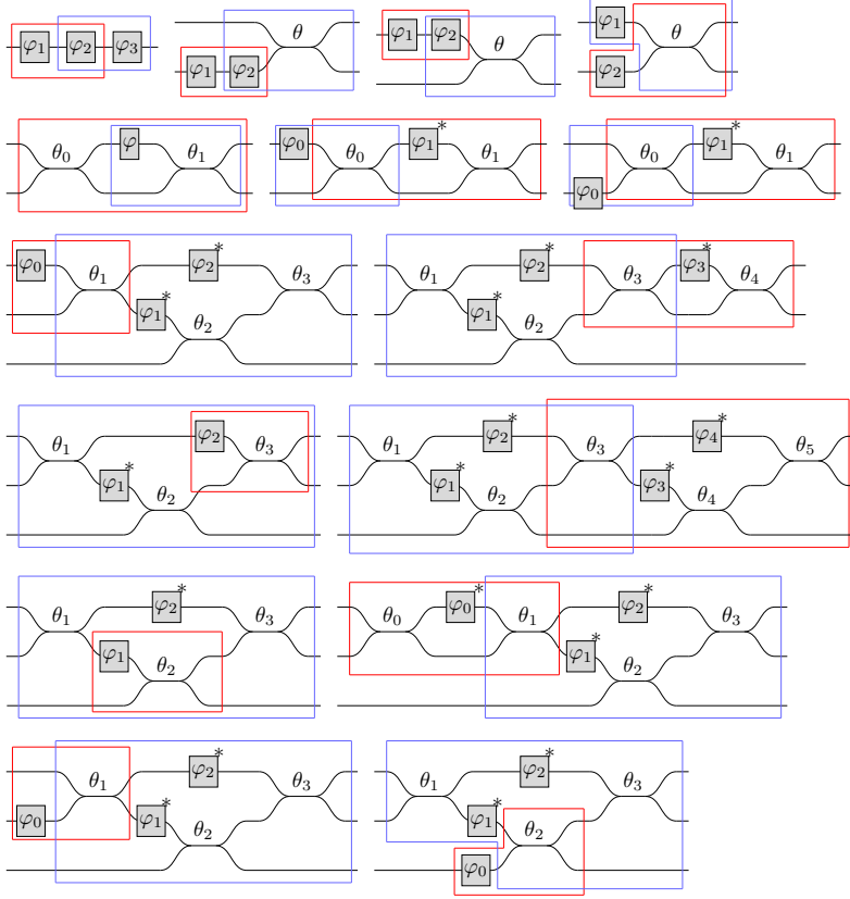
Figure 5.9: Non-trivial critical peaks (more precisely, those not involving single-generator patterns).
