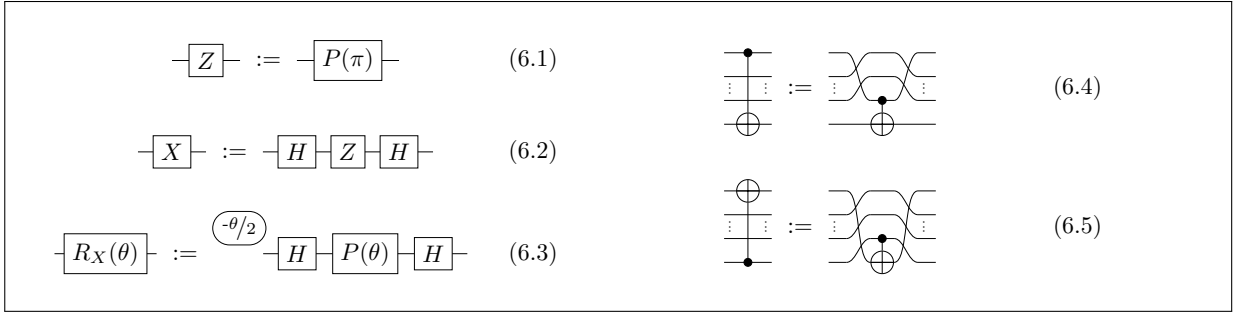
Figure 6.1: Usual abbreviations of quantum circuits.
