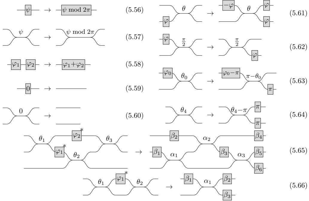
Figure 5.7: Rewriting rules of PPRS. \psi \in \mathbb{R} \setminus [0, 2\pi) , \varphi, \varphi_1, \varphi_2 \in (0, 2\pi) , \varphi_0, \theta_4 \in [\pi, 2\pi) , \theta, \theta_0, \theta_1, \theta_2, \theta_3 \in (0, \pi) , and \theta_0 \neq \frac{\pi}{2} . \boxed{\varphi}^* denotes either \boxed{\varphi} or \text{---} . In Rules (5.65) and (5.66), the angles on the left-hand side can take any value while the right-hand side is given by Lemma 5.13 and Lemma 5.12 respectively.
