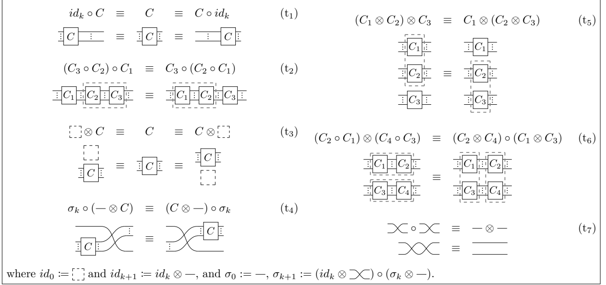
Figure 6.5: Definition of \equiv for raw circuits (either raw quantum circuits or raw optical circuits). Here the symbol \otimes stands for either \otimes or \oplus .
