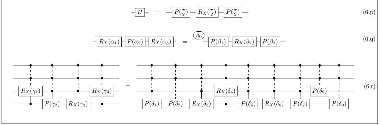
Figure 6.4: Non-structural equations. In Equations (6.q) and (6.r) the LHS circuit has arbitrary parameters which uniquely determine the parameters of the RHS circuit. Equation (6.q) is nothing but the well-known Euler-decomposition rule which states that any unitary can be decomposed, up to a global phase, into basic X - and Z -rotations. Thus for any \alpha_i \in \mathbb{R} , there exist \beta_j \in \mathbb{R} such that Equation (6.q) is sound. We make the angles \beta_j unique by assuming that \beta_1 \in [0, \pi) , \beta_0, \beta_2, \beta_3 \in [0, 2\pi) and if \beta_2 \in \{0, \pi\} then \beta_1 = 0 . Equation (6.p) is the particular Euler decomposition of H . Equation (6.r) reads as follows: the equation is defined for any n \geq 2 input qubits, in such a way that all gates are controlled by the first n-2 qubits. Equation (6.r) can be seen as a generalisation of the Euler rule, using multi-controlled gates. Similarly to Equation (6.q), for any \gamma_i \in \mathbb{R} , there exist \delta_j \in \mathbb{R} such that Equation (6.r) is sound. We ensure that the angles \delta_j are uniquely determined by assuming that \delta_1, \delta_2, \delta_5 \in [0, \pi) , \delta_3, \delta_4, \delta_6, \delta_7, \delta_8, \delta_9 \in [0, 2\pi) , if \delta_3 = 0 then \delta_2 = 0 , if \delta_3 = \pi then \delta_1 = 0 , if \delta_4 = 0 then \delta_1 = \delta_3 (= \delta_2) = 0 , if \delta_4 = \pi then \delta_2 = 0 , if \delta_4 = \pi and \delta_3 = 0 then \delta_1 = 0 , and if \delta_6 \in \{0, \pi\} then \delta_5 = 0 .
