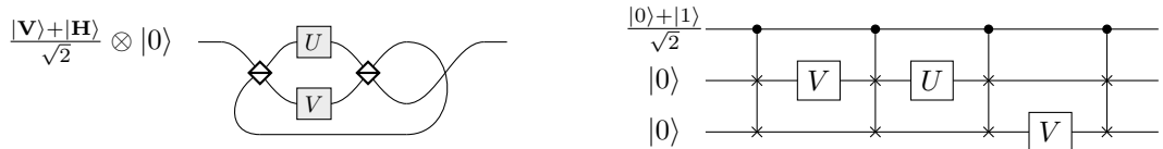
Figure 4.1: [Left] Coherently controlled quantum computation for solving the commuting problem. Only two queries are used: one query to U and one query to V . [Right] Optimal circuit for solving the commuting problem, where the 3-qubit gate is a control-swap. Note that three queries are necessary in the quantum circuit model.
