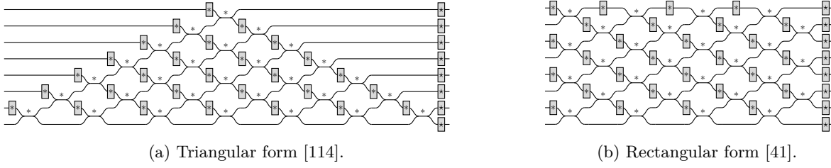
Figure 5.1: Triangular and rectangular universal forms for polarisation-preserving circuits.
