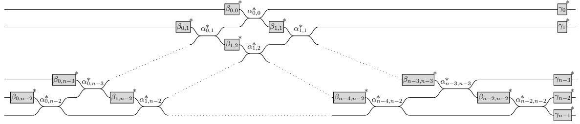
Figure 5.10: General scheme of a PPRS triangular normal form. The stars mean that any phase shifter or beam splitter with angle 0 is replaced by the identity. The conditions on the angles are the following: \alpha_{i,j}, \beta_{i,j} \in [0, \pi) ; \gamma_i \in [0, 2\pi) ; \alpha_{i,j} = 0 \Rightarrow \forall j' > j, \alpha_{i,j'} = 0 ; \alpha_{i,j} \in \{0, \frac{\pi}{2}\} \Rightarrow \beta_{i,j} = 0 .
