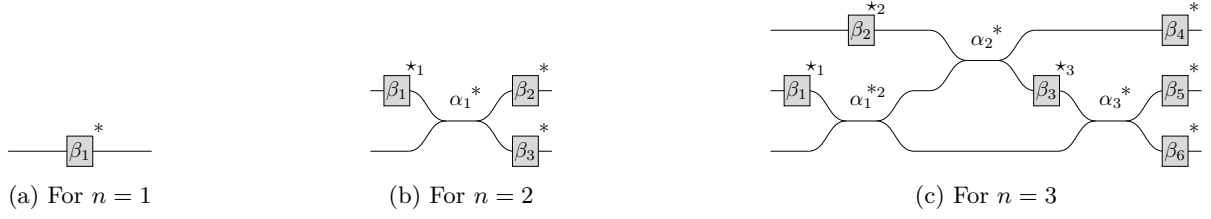
Figure 5.8: Normal forms of PPRS for n \in \{1, 2, 3\} . * means that the phase shifter or beam splitter is replaced by (an) identity wire(s) when the angle is zero. *_i represents the identity in the preceding case and also when \alpha_i = 0 . \star_i represents the identity in the preceding two cases and also when \alpha_i = \frac{\pi}{2} . The \alpha_i are in [0, \pi) as well as the phases with a \star_i , all other phases are in [0, 2\pi) .
