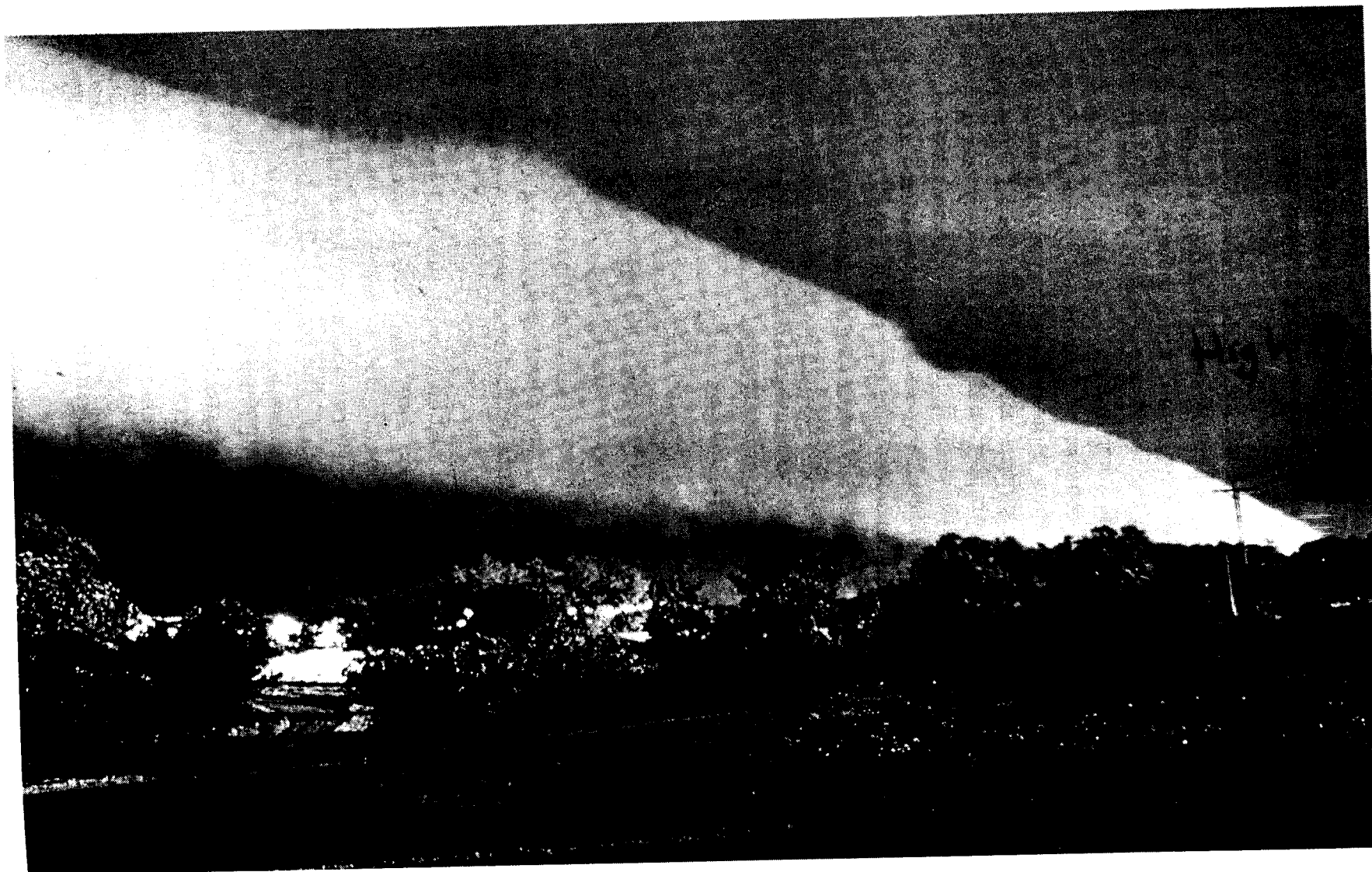
Fig. 9.3 An arcus cloud marking a gust front emanating from a thunderstorm over Oklahoma. (Photo courtesy of Howard Bluestein.)
