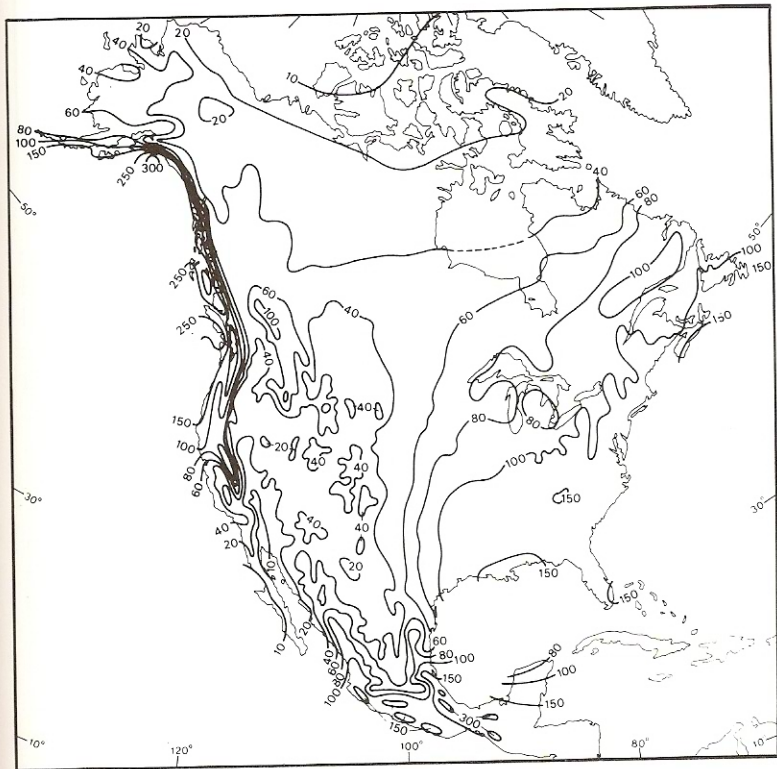
Figure 5.20 Mean annual precipitation (in centimetres) over North America for the period 1931–60. Isohyets in the Arctic underestimate the true totals by 30–50 per cent due to problems in recording snowfall accurately with precipitation gauges.
