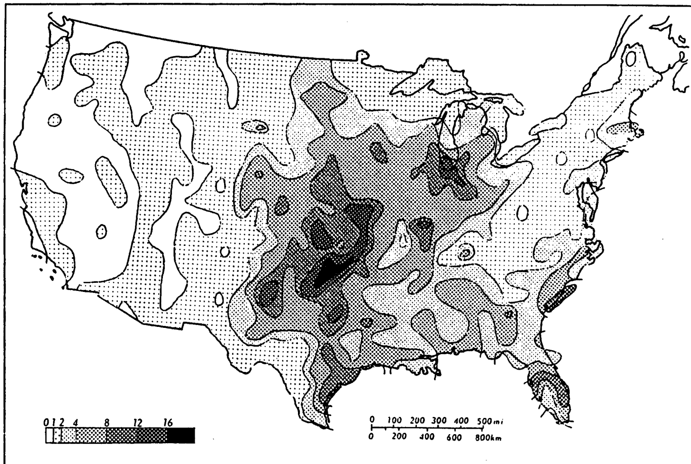
Fig. 9.7 Mean annual incidence of tornadoes per 2.6 \times 10^4 \text{ km}^2 , 1955–67. [From Bryson and Hare (1974).]
