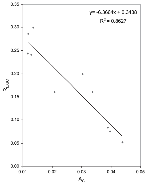
FIG. 1.—Negative relationship between A_C (selection against C usage) and R_{L,GC} (correlation between the length and GC% of CDSs) in 10 Chlamydiae/Verrucomicrobia genomes.
